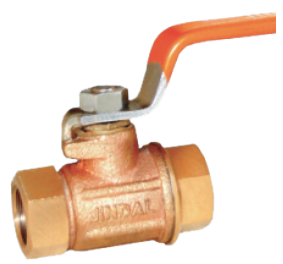
G.M. Ball Valves (Heavy) with Brass/SS Part & Teflon Seat Hyd. Tested 300 lbs. Size : 15mm to 100mm
